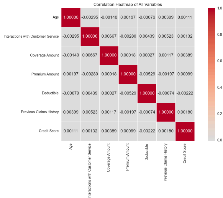
Gambar 4.5 Heatmap Correlation
