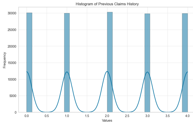
Gambar 4.2 Histogram Variabel Previous Claims History
